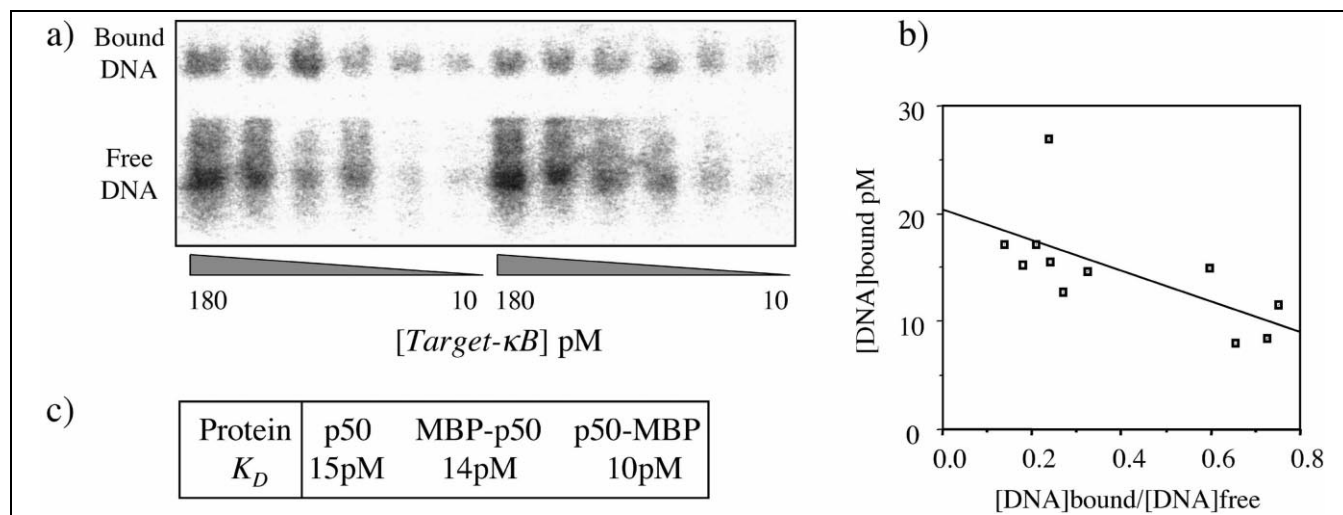
Fig. 2. Gel shift (a) and Scatchard (b) analysis of the fusion protein MBP-p50 binding to an oligonucleotide containing the sequence target-kB . c: Calculated equilibrium binding constants for each protein binding to the target-kB sequence.
